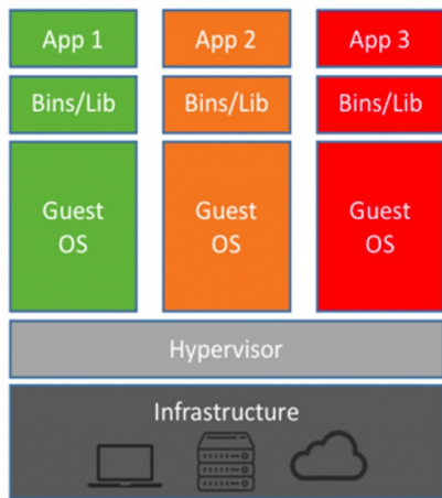
Machine Virtualization
